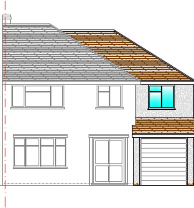
Front Elevation
